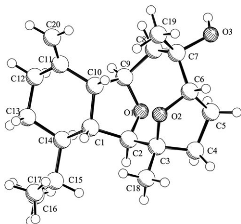
Figure 1. Solid-state structure of (+)-1. [34–36]
