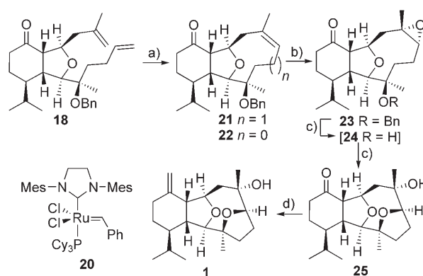
Scheme 5. Metathesis and completion of the total synthesis of (+)-vigulariol ( 1 ). Reagents and conditions: a) 20 (10 mol%), benzene, reflux, 1.3 h, 45% 21 , 17% 22 ; b) 1.1 equiv \text{DMDO} , acetone, -20^\circ\text{C} , 30 min, 81% 23 , 9% \alpha - 23 ; c) 10% \text{Pd/C} (20 mol%), \text{H}_2 (1 bar), \text{EtOAc} , 22^\circ\text{C} , 1.25 h, 91%; d) 4.0 equiv \text{Ph}_3\text{PCH}_2\text{Br} , 3.5 equiv \text{NaHMDS} (1 M in THF), toluene, 80^\circ\text{C} , 45 min, 93%. \text{DMDO} = dimethyldioxirane, \text{NaHMDS} = sodium hexamethyldisilazide, Cy = cyclohexyl, Mes = 2,4,6-trimethylphenyl.
