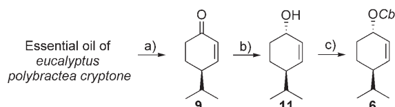
Scheme 2. Preparation of carbamate 6 . Reagents and conditions: a) Flash column chromatography (FCC), 12.6 g 9 (97% ee); C15-sesquiterpene in a ratio of 47:53 (GC) from essential oil (100 mL); b) 1.2 equiv \text{LiAlH}_4 , \text{Et}_2\text{O} , -78^\circ\text{C} , 30 min, FCC, 5.27 g (37.6 mmol) 11 (d.r. = 84:16); c) 1.2 equiv \text{NaH} , 1.4 equiv i\text{Pr}_2\text{NC(O)Cl} , THF, reflux, 12 h, FCC, 78% 6 (97% ee), 12% cis - 6 .
