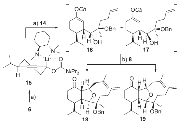
Scheme 4. Synthesis of the metathesis precursor 18 by a homoaldol reaction and THF cyclocondensation. Reagents and conditions: a) 1) 1.05 equiv s\text{BuLi} /TMCD, \text{Et}_2\text{O} , -78^\circ\text{C} , 2 h; 2) 1.74 equiv \text{ClTi}(\text{OiPr})_3 (1.74 M in toluene), -78^\circ\text{C} , 2 h; 3) 2.5 equiv 14 , -78^\circ\text{C} to 22^\circ\text{C} , 13.5 h, 16/17 (d.r. = 83:17, 40% from 6 ), 69% 14 reisolated; b) 2.1 equiv 8 , 1.9 equiv \text{BF}_3 \cdot \text{OEt}_2 , \text{Et}_2\text{O} , 0^\circ\text{C} , 35 min; 71% 18 , 13% 19 (from 16/17 83:17). TMCD = rac-trans - N,N,N',N' -tetramethyl-1,2-diaminocyclohexane.
