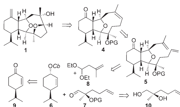
Scheme 1. Retrosynthetic analysis of (+)-vigulariol ( 1 ). Cb = C(O)NiPr 2 , PG = protecting group.
